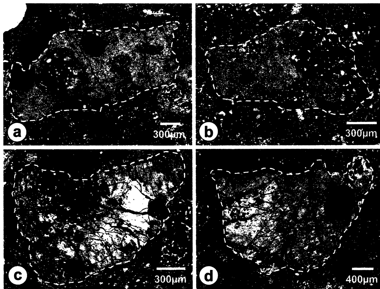
FIG. 1. Backscattered electron images of dark inclusions (DIs; outlined by white broken lines) in the Mokoia CV3 chondrite. (a) DI-1. (b) DI-2. (c) DI-3. (d) DI-4. The DIs are distinctly brighter relative to the host meteorite. DI-3 and DI-4 have high densities of fractures; most of them terminate at the boundary between the DIs and the host meteorite.
