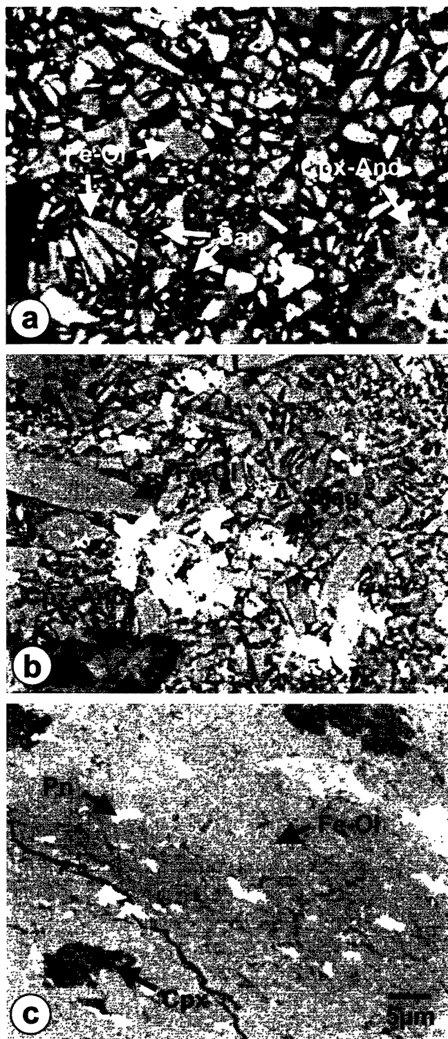
FIG. 5. Backscattered electron images of matrices in Mokoia host (a), DI-1 (b), and DI-3 (c). All the images are at the same magnification. Fe-Ol = Fe-rich olivine. Sap = saponite. Cpx = Ca-Fe-rich clinopyroxene. And = andradite. Mag = magnetite. Pn = pentlandite.
