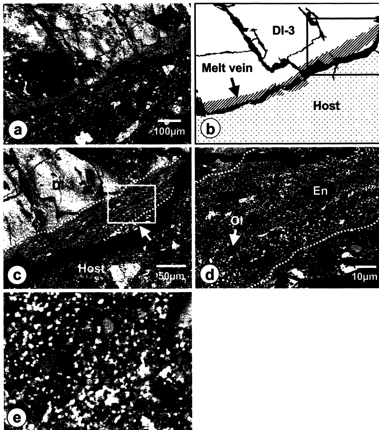
FIG. 10. (a) Backscattered electron image of a melt vein in DI-3. The vein is located along an edge of the DI. (b) Illustration of the image in (a). (c) Image of boxed area in (b), showing a portion of the melt vein. Note that a small lenticular area (indicated by a white arrow) having the same lithology as the DI matrix is attached to the vein. (d) Image of boxed area in (c), showing that the melt vein contains fragments of olivine (Ol) and enstatite (En). (e) High-magnification image of a portion of the melt vein, showing that the vein contains numerous rounded inclusions of pentlandite and magnetite (bright particles) and rounded pores as well as fragments of Fe-rich olivine (Fe-Ol) and enstatite.
