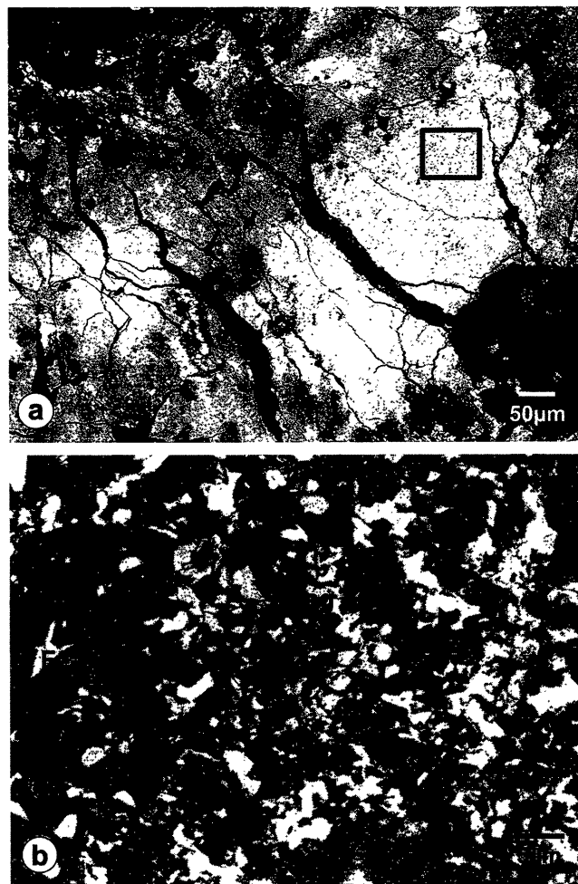
FIG. 8. (a) Backscattered electron image of a portion of DI-3 including very Fe-rich areas (bright) in matrix. (b) Low-contrast image of boxed area in (a), showing intermixed grains of Fe-rich olivine (Fe-Ol), magnetite (Mag) and pentlandite (Pn).
